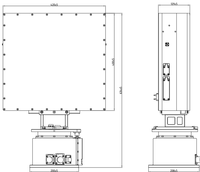
CR-PK14B structural and installation dimensions (unit: mm)
